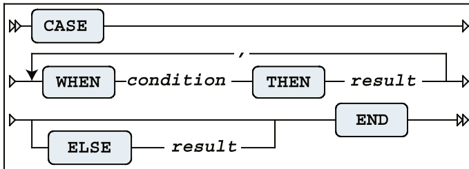
Figure 4-5. Searched CASE expressions syntax diagram
