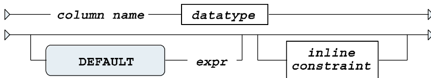
Figure 7-2. A CREATE TABLE column specification syntax
